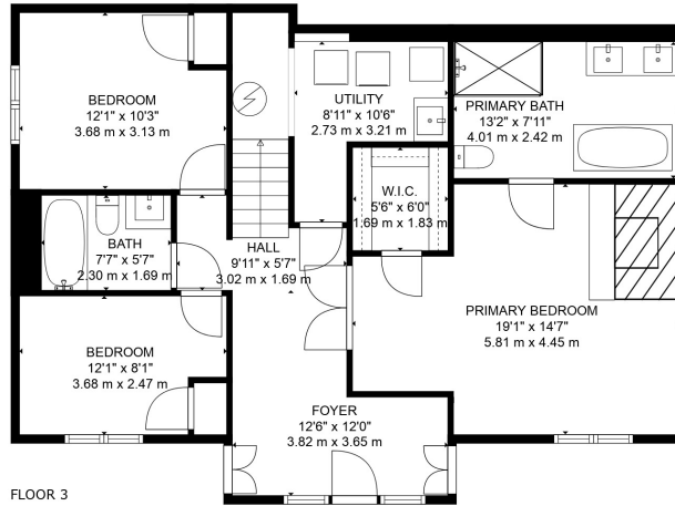
FLOOR 3
