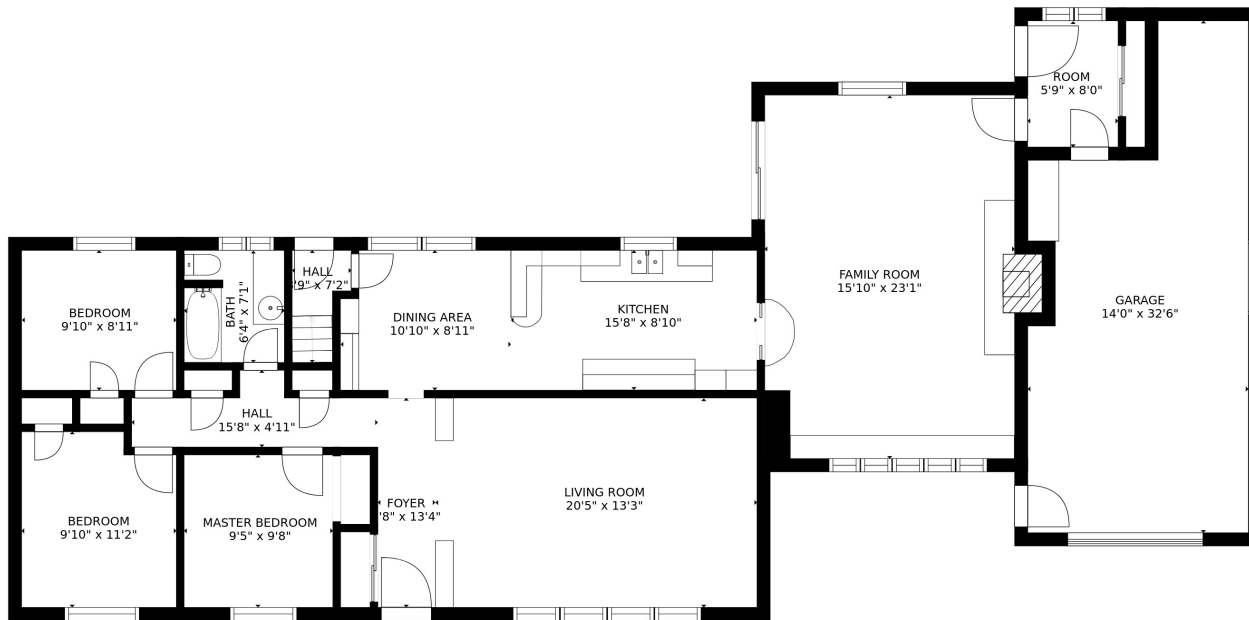
FLOOR 2
